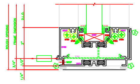
202 I.G. SILL SERIES: 403X - 2" X 4 1/2" SHEARBLOCK
