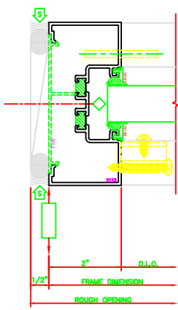
401 I.G. JAMB SERIES: 403X - 2" X 4 1/2" SHEARBLOCK
